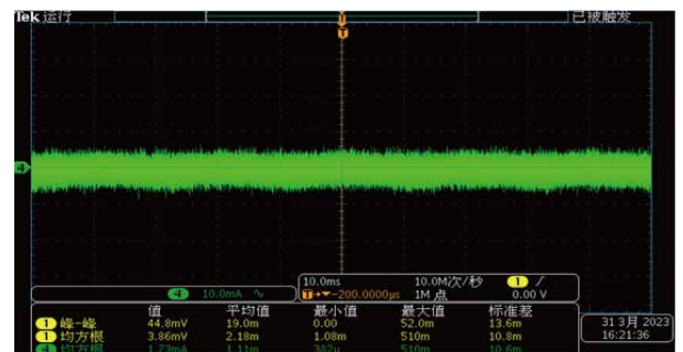
Max. ripple of IT-N2133(1.5kW) is about 10mA
