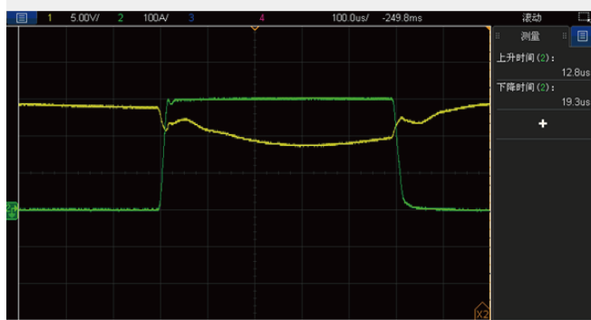
Dynamic voltage and current with low inductance test Cables
